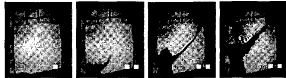
Figure 4: Exposures of 25 \mu\text{s} at t = 0, 0.5, 1.6, 3.4 \text{ msec} after a pulse of 2 \times 10^{12} protons interacted with a "thimble" of mercury 1.0 cm in diameter and 1.5 cm deep.
