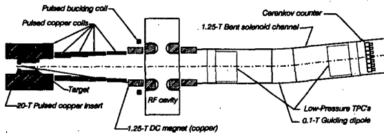
Figure 2: Sketch of the full configuration of BNL E951, the targetry R&D facility.
