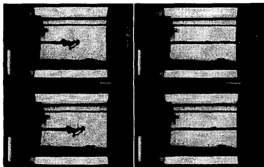
High-speed photographs of mercury jet target for CERN-PS-AA (laboratory tests) 4,000 frames per second, Jet speed: 20 ms -1 , diameter: 3 mm, Reynolds's Number: >100,000 A. Pomot
