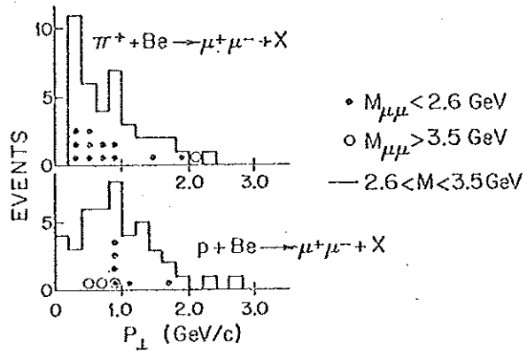
Fig. 4 p_{\perp} distributions. The acceptance is uniform in p_{\perp} within 20 percent.
