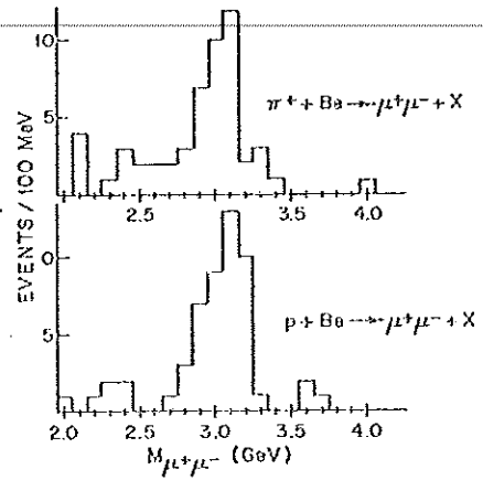
Fig. 2 Uncorrected Mass Spectra
