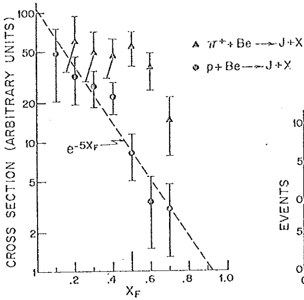
Fig. 3 Relative cross-sections for J production.
