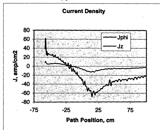
Figure 5: Induced j_\phi and j_z from the finite element calculation along mercury jet path. The current densities are calculated on the surface of the jet.
