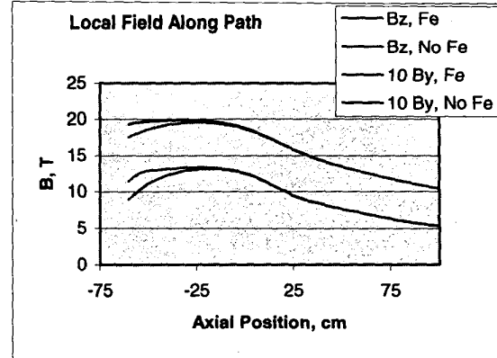
Figure 2: B_z and B_y are given as a function of the path position in the local coordinate system of the mercury jet. Curves show the field with and without the presence of a steel pole. The B_y curve is multiplied by 10 to be visible on the plot.
