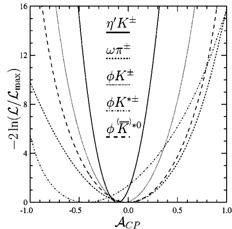
FIG. 1. Dependence of \chi^2 \equiv -2 \ln(\mathcal{L}/\mathcal{L}_{\text{max}}) on \mathcal{A}_{CP} for each of the B decay modes.
