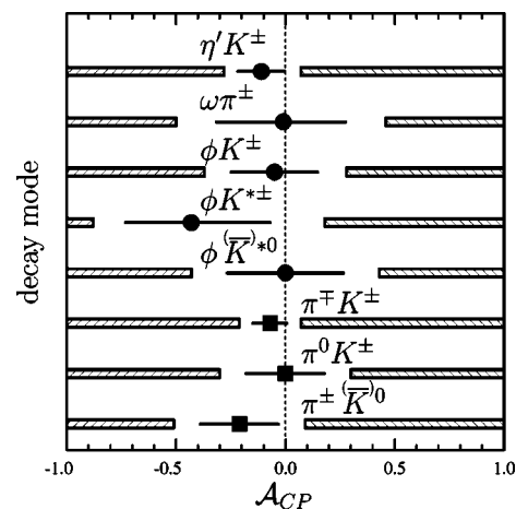
FIG. 2. Results of \mathcal{A}_{CP} measurements for the B decay modes presented in this paper (circles) with the BABAR measurements in \pi K modes (squares) shown for comparison [10,11]. The data sample for the \pi^\mp K^\pm result is about 50% larger [11]. Hatched regions are excluded at 90% C.L.
