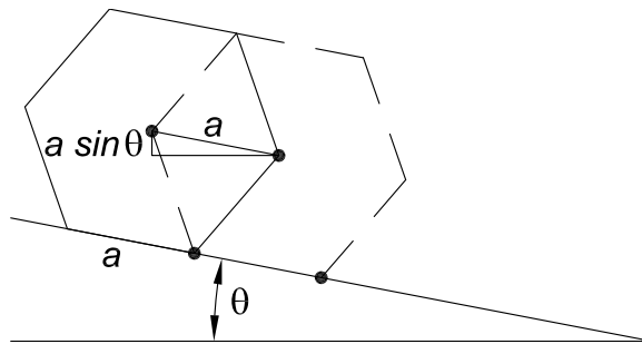
Figure 2: The center of mass of a hexagonal pencil falls through height a \sin \theta during each 1/6 turn, where a is the width of a face of the pencil. For an N -sided pencil whose faces have width b , the center of mass falls by b \sin \theta during each 1/N turn.
