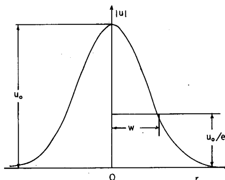
FIG. 1. Amplitude distribution of a Gaussian beam.
