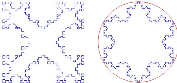
Figure 1: Two examples of the pattern of the conductor in fractal loop antennas.
