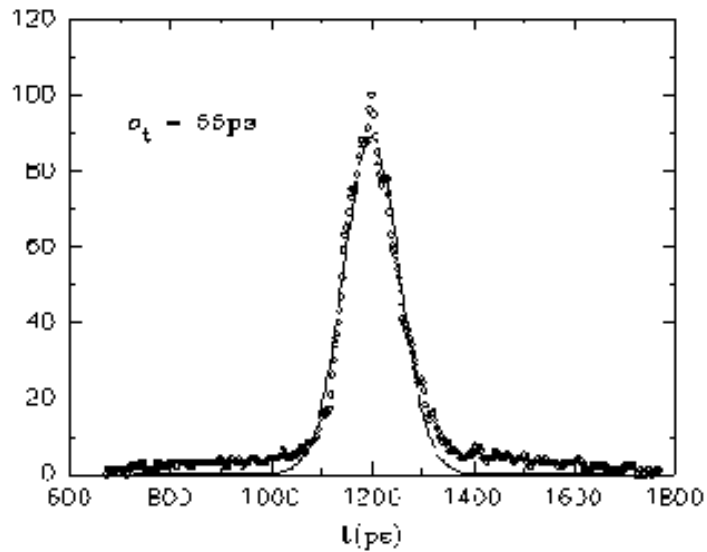
Figure 2: The time resolution of two Hamamatsu R3809U MCP-PMT's as determined with the setup shown in Fig. 1. The joint distribution was observed to have \sigma = 55 ps, corresponding to \sigma = 39 ps for each MCP-PMT.
