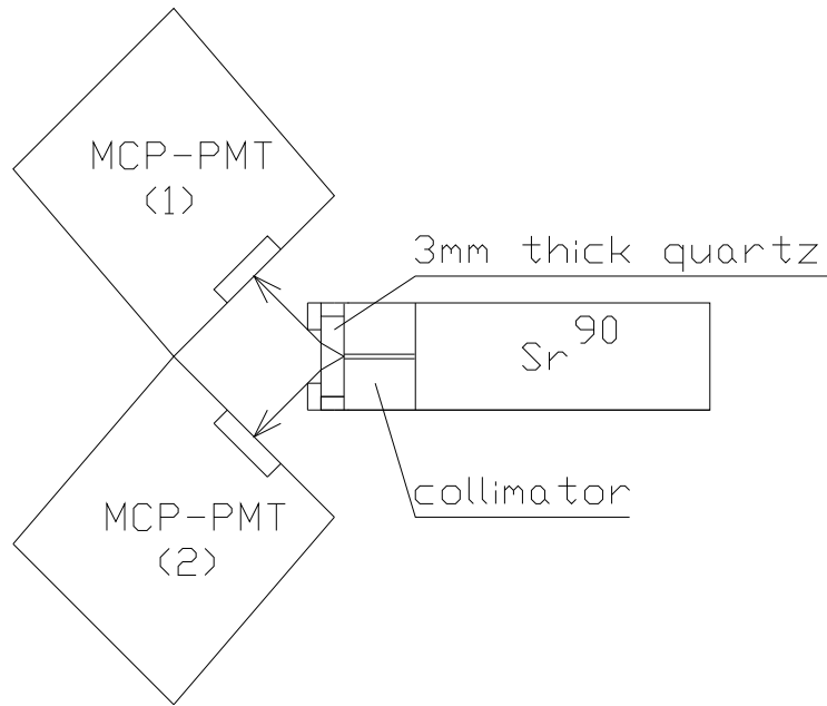
Figure 1: Setup to measure the time resolution of a pair of Hamamatsu R3809U MCP-PMT's.
